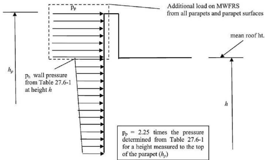
FIGURE 27.5-2 Main Wind Force Resisting System, Part 2 [ h \leq 160 ft ( h \leq 48.8 m)]: Enclosed Simple Diaphragm Buildings, Parapet Wind Loads.
