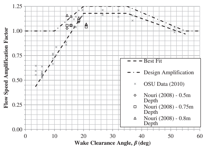
FIGURE C6.8-4 Amplification of Flow Speed vs. Wake Clearance Angle
