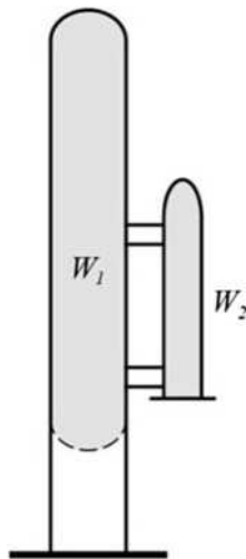
FIGURE C15.1-7 Torsional irregularity
