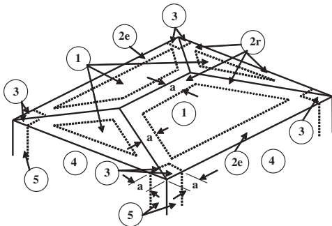
Hip Roof: 7 \leq \theta \leq 45 degrees; h \leq 160 ft
