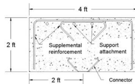
FIGURE C14.2-4 Test Module
