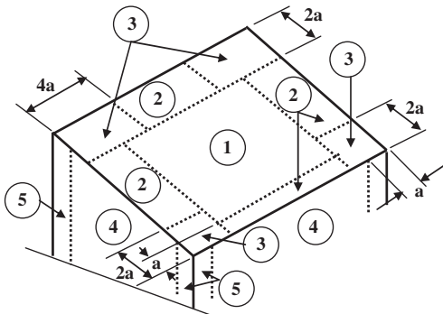
Monoslope Roof: 7 < \theta \leq 30 degrees; h \leq 160 ft
