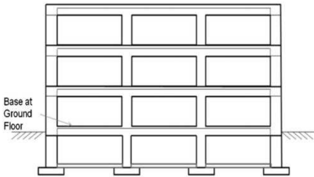
FIGURE C11.2-3 Base at Ground Floor Level
