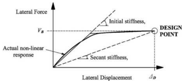
FIGURE C6.11-1 Stiffness Definitions for Initial Elastic and Effective Secant Stiffness
