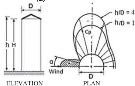
FIGURE 30.12-1 Components and Cladding [ h \leq 120 ft ( h \leq 36.6 m)]: External Pressure Coefficients, ( GC_p ), for Walls of Isolated Circular Bins, Silos, and Tanks with D < 120 ft (36.6 m) and 0.25 < H/D < 4.0 —Other Structures
