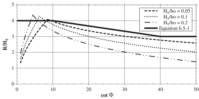
FIGURE C6.5-1 Runup Ratio R/H_T , as a Function of the Mean Slope of the Nearshore Profile, \cot \Phi for Relative Wave Heights H_T/h_o = 0.05, 0.1, \text{ and } 0.2
