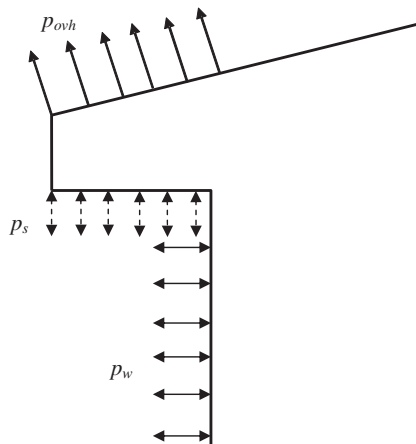
FIGURE 30.9-1 Components and Cladding (All Building Heights): Wind Loading on Roof Overhangs for All Building Types—C&C Wind Loads on Roof Overhangs
