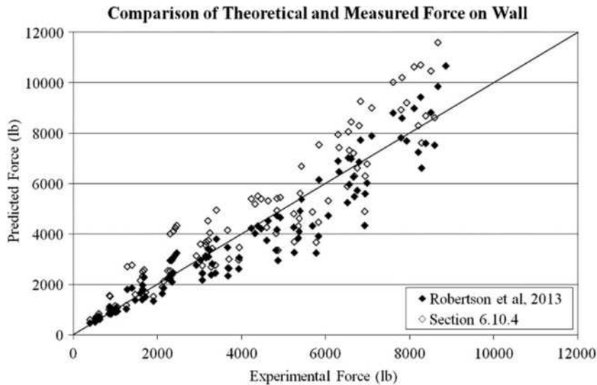
FIGURE C6.10-1 Predicted vs. Experimental Bore Loading on Wall (1:5 Model Scale)
