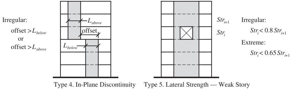
FIGURE C12.3-2 Vertical Structural Irregularities
