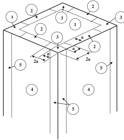
Flat Roof: \theta \leq 7 degrees; h > 60 ft
