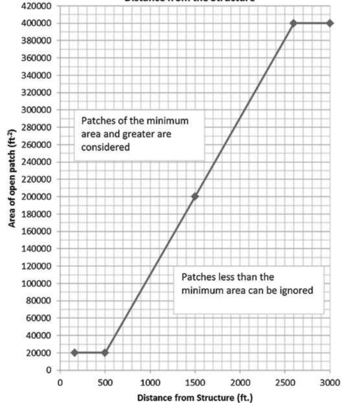
FIGURE C26.7-4 Minimum Area of Individual Open Patches Affecting Qualification of Exposure B
