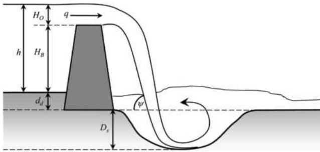
FIGURE 6.12-2 Plunging Scour Parameters
