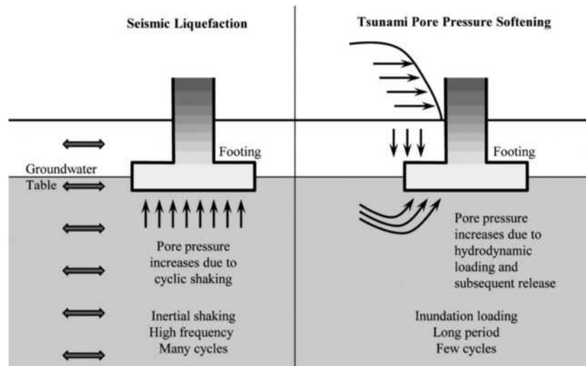
FIGURE C6.12-2 Schematic Diagram Showing Differences between Seismic Liquefaction and Tsunami-Induced Pore Pressure Softening
