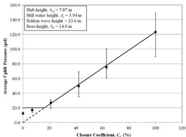
FIGURE C6.10-4 Mean Slab Uplift Pressure Reduction Caused by Perforated Wall (1 psf = 0.048 kPa; 1 in. = 25.4 mm)
