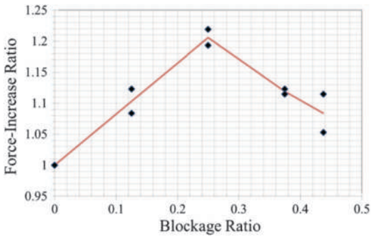
FIGURE C6.8-2 Flow Amplification Force-Increase Ratio for Channelized Conditions (Where the Blockage Ratio Is the Net Width of Constricting Obstructions Divided by the Total Flume Width)
