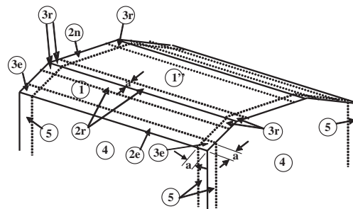
Mansard Roof: 7 \leq \theta \leq 45 degrees; h \leq 160 ft (See Note 2)
