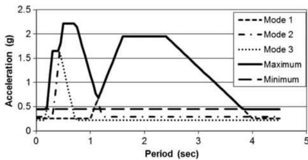
FIGURE C13.3-3 Approximate Floor Response Spectrum
