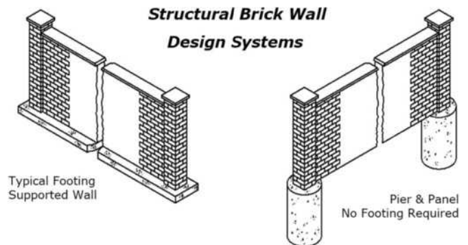
FIGURE C15.6-3 Typical Cantilever Wall Systems Falling under the Requirements of Section 15.6.8.
