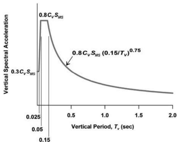
FIGURE C11.9-1 Illustrative Example of the Vertical Response Spectrum
