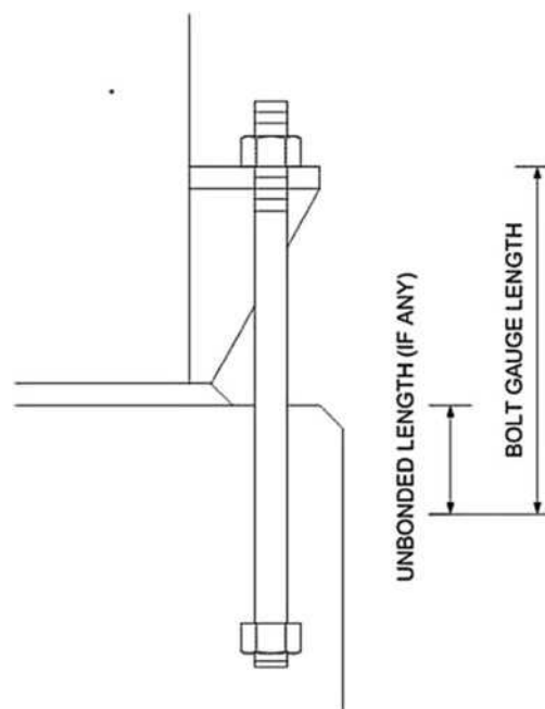
FIGURE C15.7-1 Bolt gauge length
