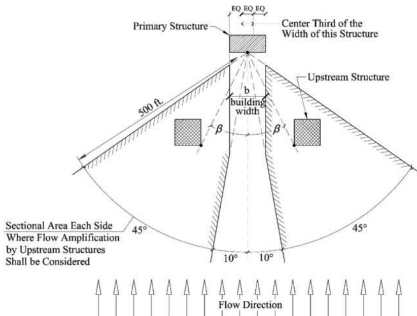
FIGURE C6.8-3 Effective Wake Clearance Angle, \beta , for Flow Amplification
