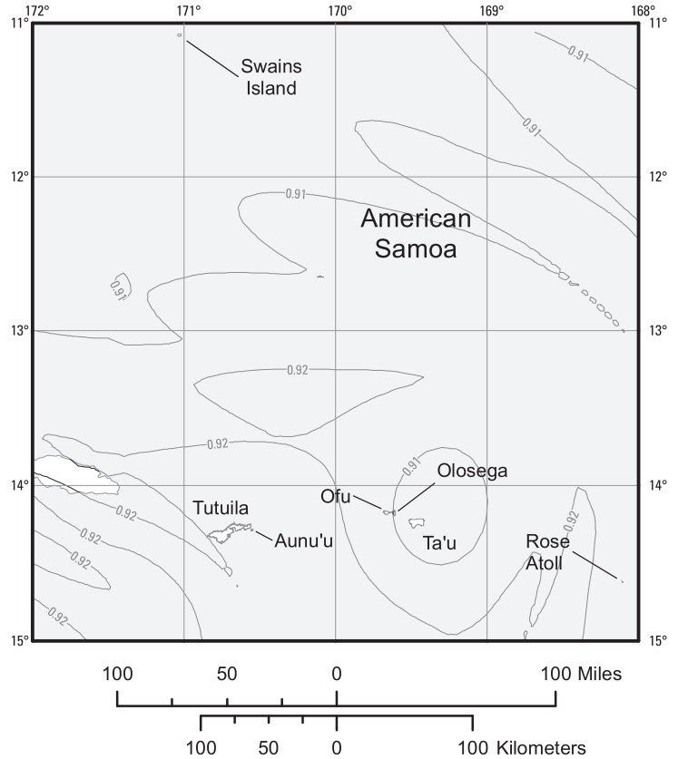
FIGURE 22-19B (Continued) Mapped Risk Coefficient at 1.0-s Spectral Response Period, C_{R1} : Guam and Northern Mariana Islands (left) and American Samoa (right)
