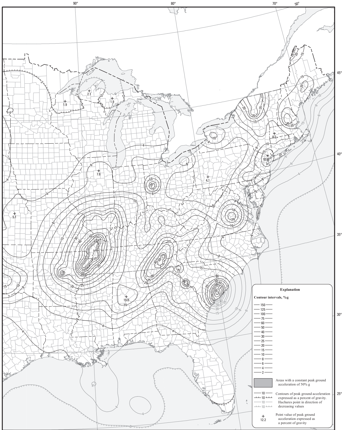
FIGURE 22-9 (Continued). Maximum Considered Earthquake Geometric Mean (MCE G ) PGA, %g, for the Conterminous United States
