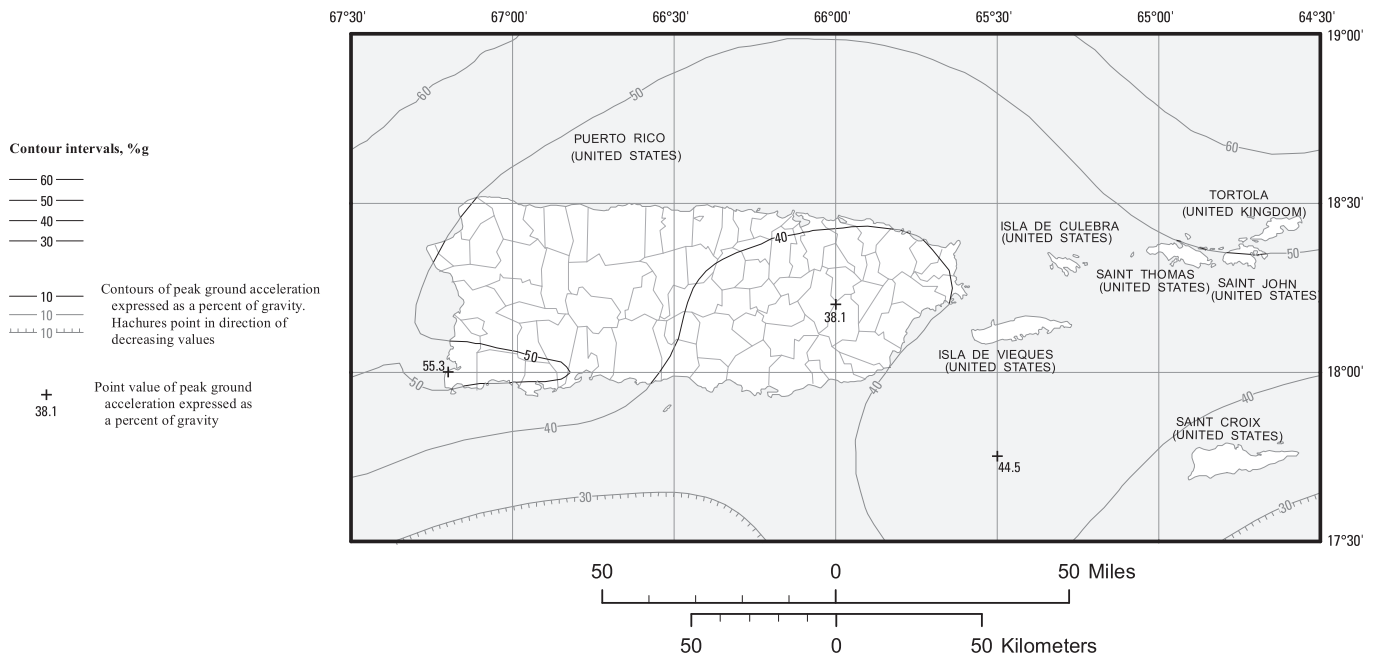
FIGURE 22-12 Maximum Considered Earthquake Geometric Mean ( MCE_G ) PGA for Puerto Rico and the U. S. Virgin Islands
