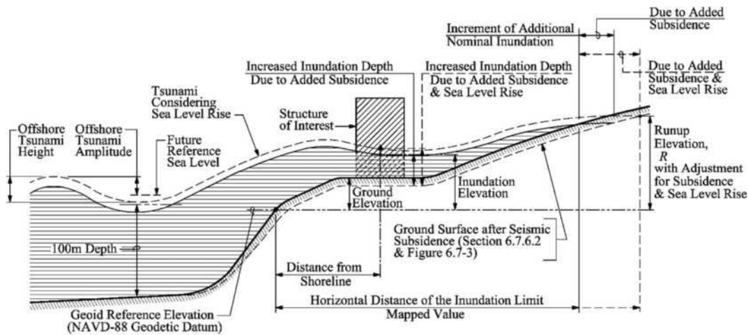
FIGURE C6.1-2 Effects of Relative Sea Level Change and Regional Seismic Subsidence on Tsunami Inundation
