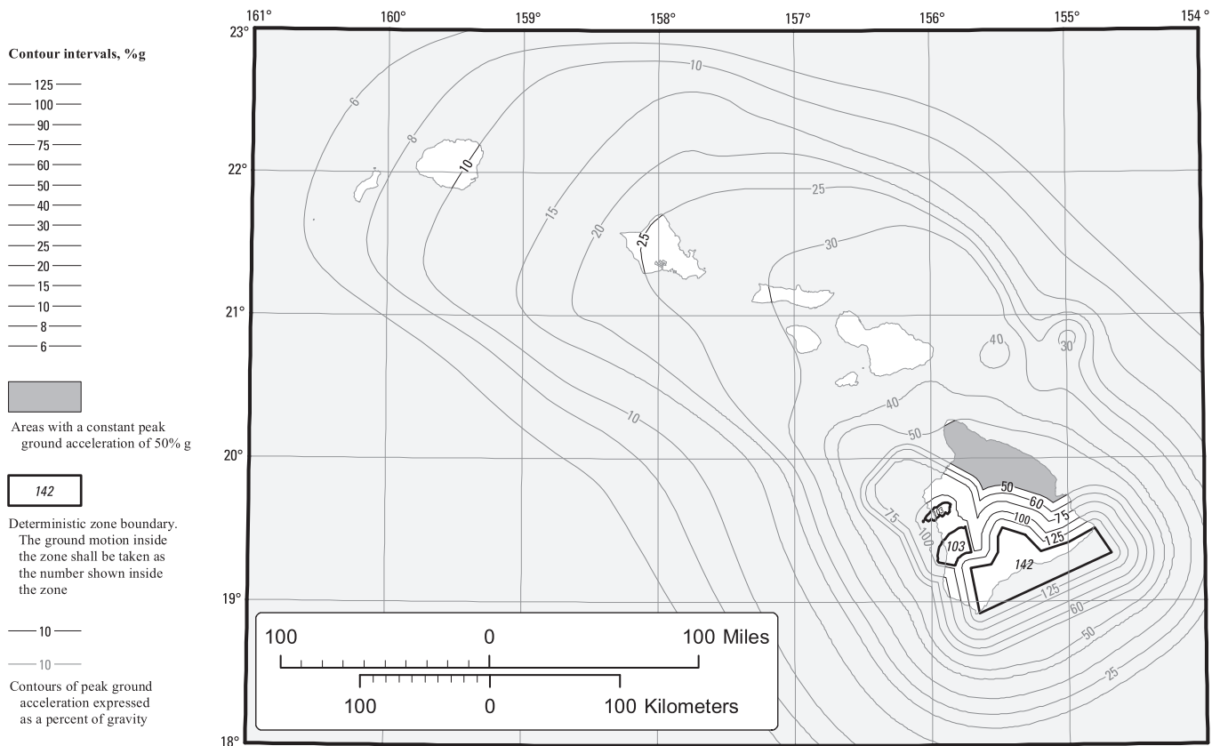
FIGURE 22-11 Maximum Considered Earthquake Geometric Mean (MCE G ) PGA for Hawaii
