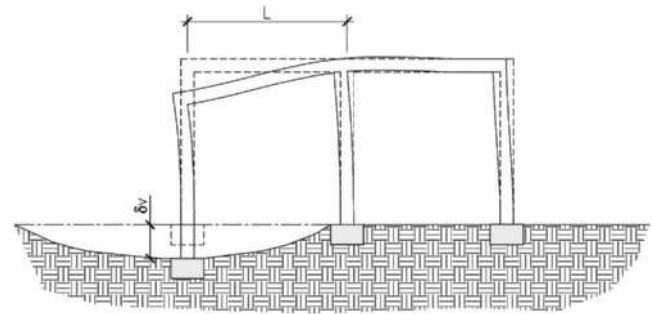
FIGURE C12.13-1 Example Showing Differential Settlement Terms \delta_v and L
