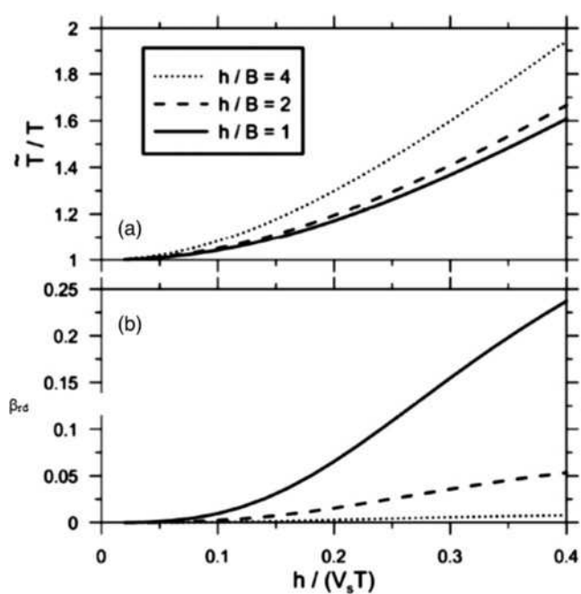
FIGURE C19.3-1 Example of Radiation Damping
