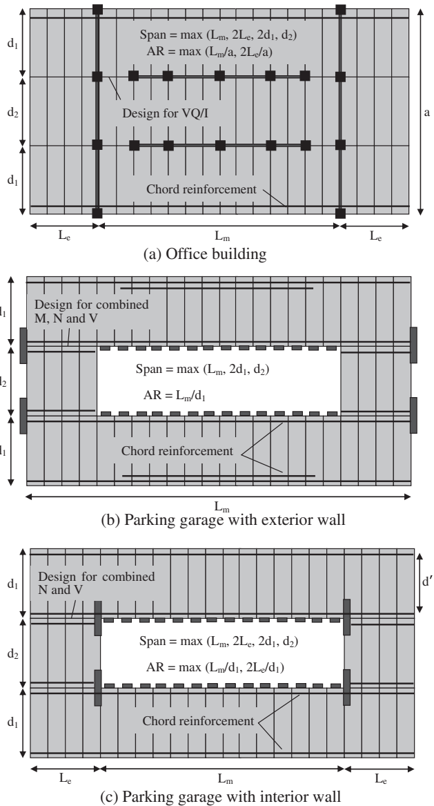
FIGURE C14.2-1 Diaphragm Dimensions
