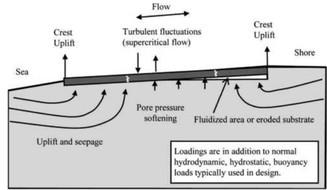
FIGURE C6.12-3 Schematic of Tsunami-Induced Loading on Exterior Slabs On Grade
