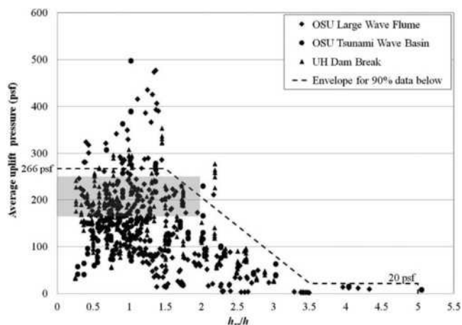
FIGURE C6.10-3 Average Uplift Pressure on Slab Soffit When Flow Is Blocked by a Solid Wall (1 psf = 0.048 kPa)
