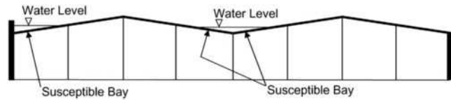
FIGURE C8.4-1 Susceptible Bays for Ponding Evaluation
