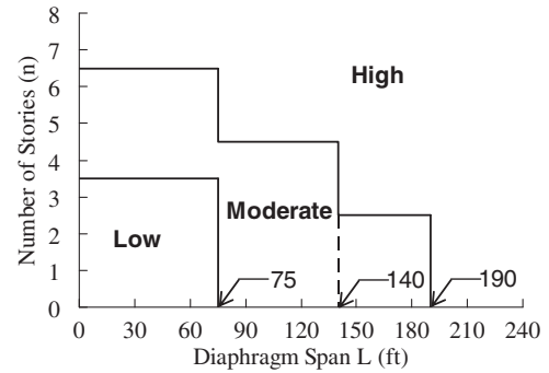
FIGURE 14.2-1 Diaphragm Seismic Demand Level
