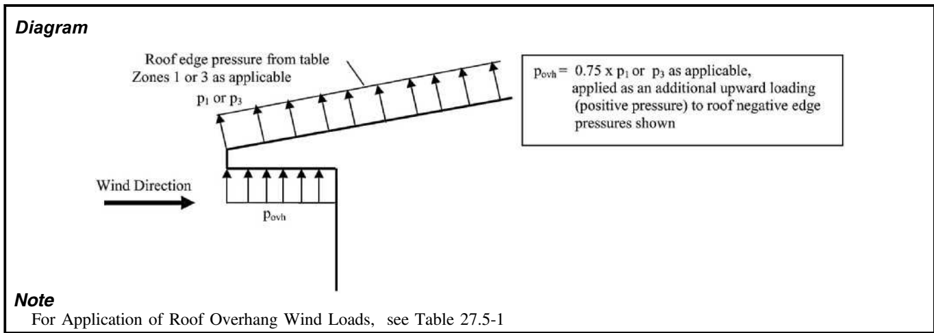
FIGURE 27.5-3 Main Wind Force Resisting System, Part 2: Enclosed Simple Diaphragm Buildings, Roof Overhang Wind Loads
