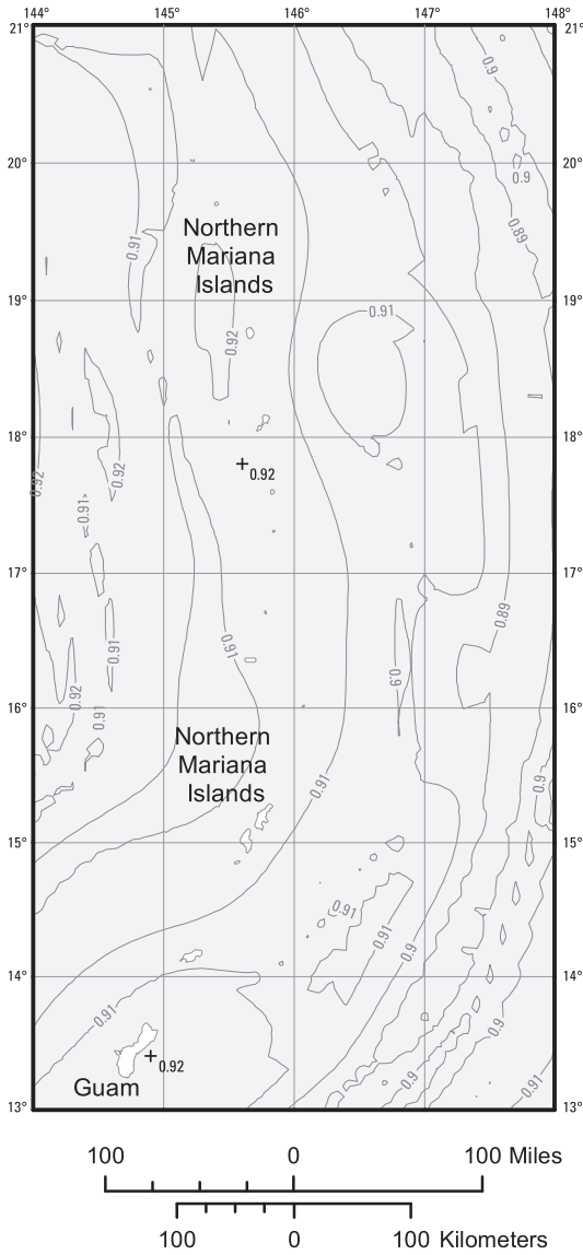
FIGURE 22-19B (Continued) Mapped Risk Coefficient at 1.0-s Spectral Response Period, C_{R1} : Guam and Northern Mariana Islands (left) and American Samoa (right)
