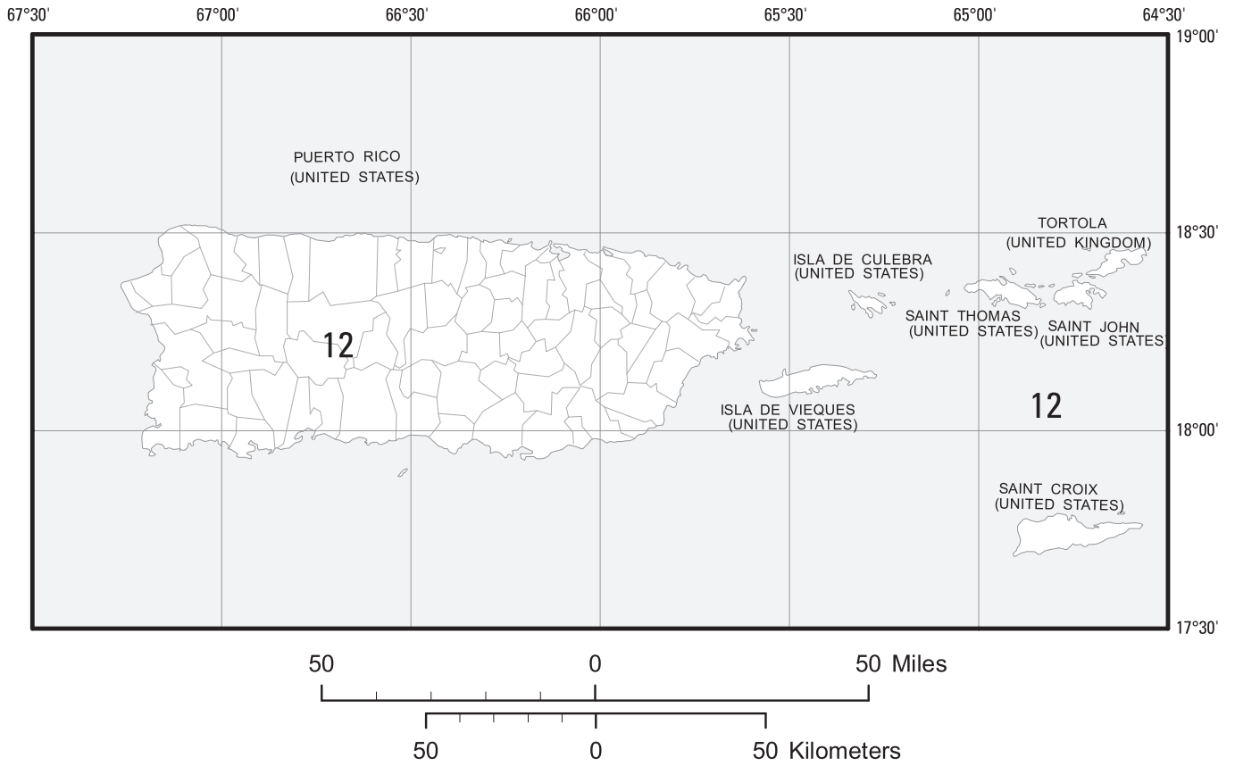
FIGURE 22-17 Mapped Long-Period Transition Period, T_L (s), for Puerto Rico and the U.S. Virgin Islands
