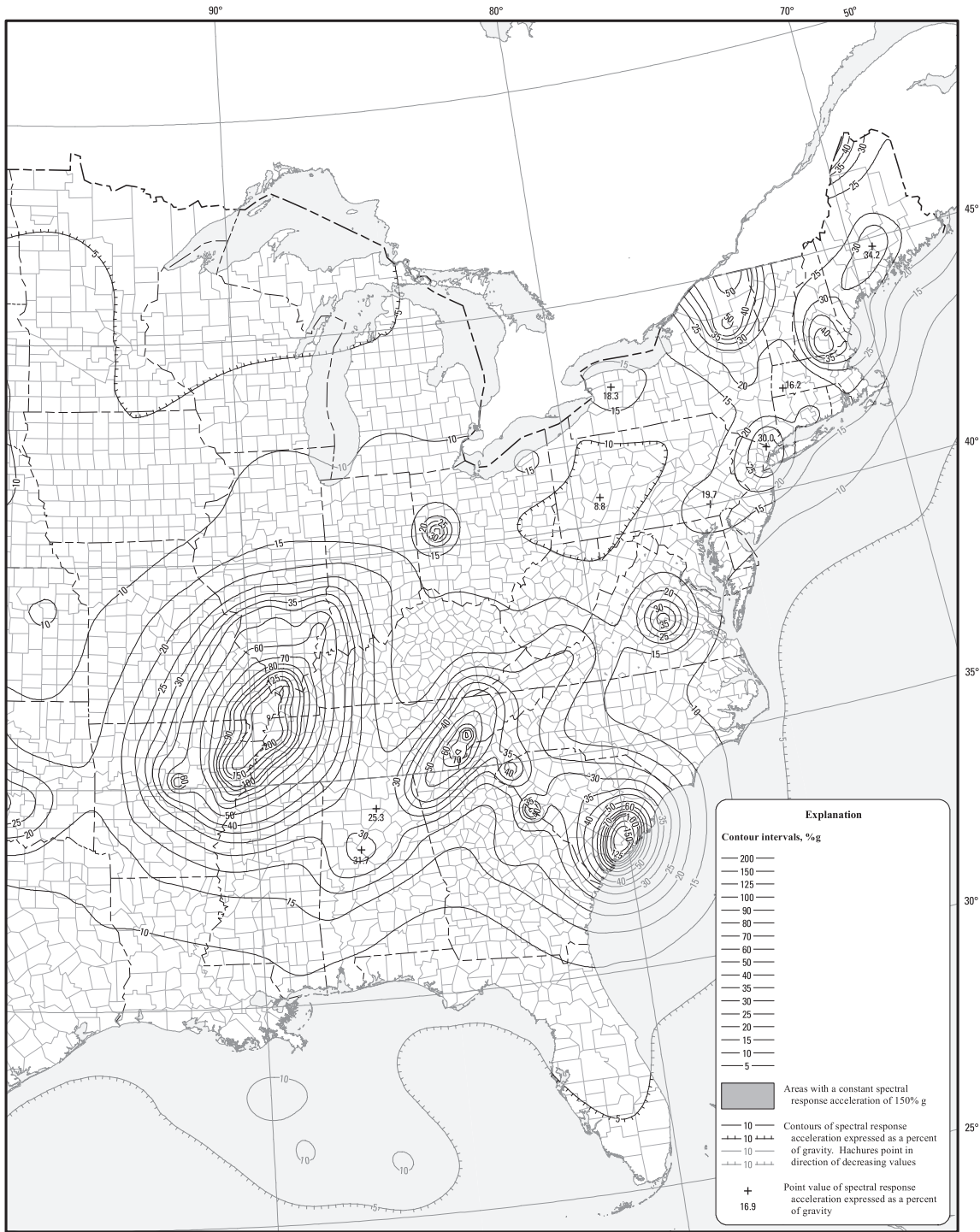
FIGURE 22-1 (Continued). S_S Risk-Targeted Maximum Considered Earthquake ( MCE_R ) Ground Motion Parameter for the Conterminous United States for 0.2-s Spectral Response Acceleration (5% of Critical Damping)
