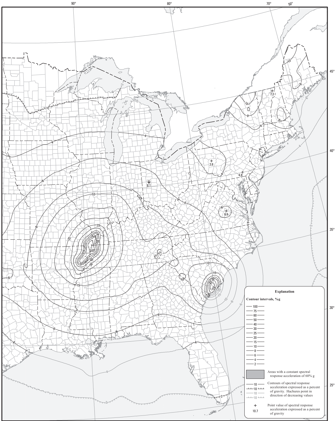
FIGURE 22-2 (Continued). S_1 Risk-Targeted Maximum Considered Earthquake ( MCE_R ) Ground Motion Parameter for the Conterminous United States for 1.0-s Spectral Response Acceleration (5% of Critical Damping)
