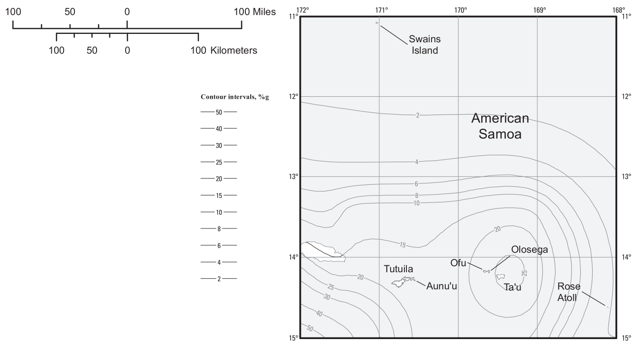
FIGURE 22-13 Maximum Considered Earthquake Geometric Mean ( MCE_G ) PGA for Guam and the Northern Mariana Islands (top) and for American Samoa (bottom)
