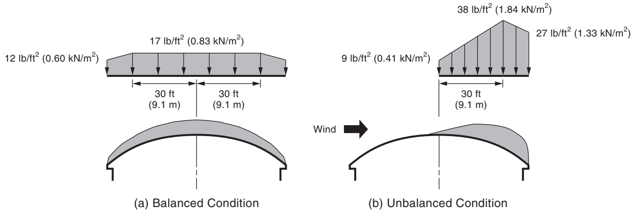
FIGURE C7.14-2 Design Snow Loads for Example 2
