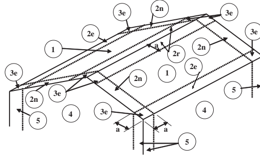
Gable Roof: 7 < \theta \leq 45 degrees; h \leq 160 ft
