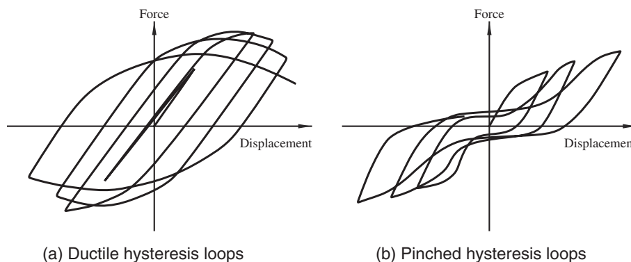
FIGURE C12.2 Typical Hysteretic Curves
