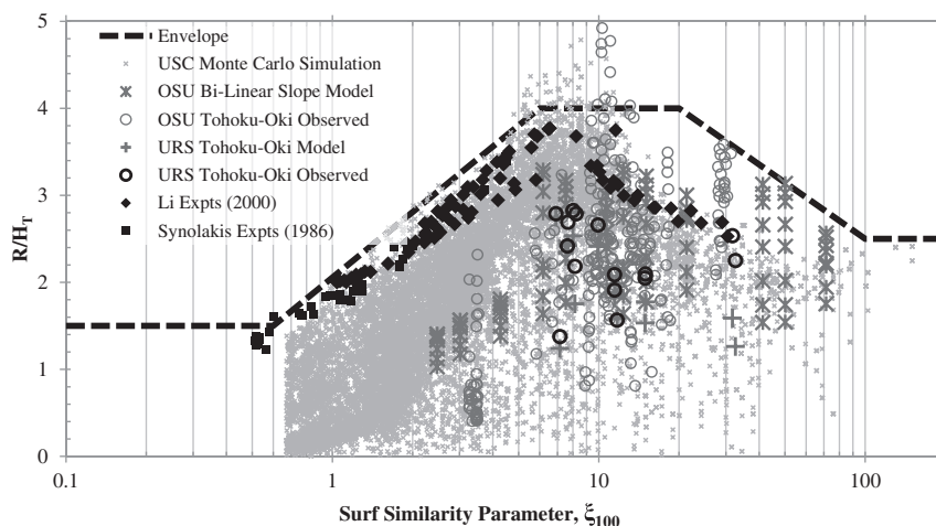
FIGURE C6.5-3 Runup Ratio R/H_T as a Function of Surf Similarity Parameter
