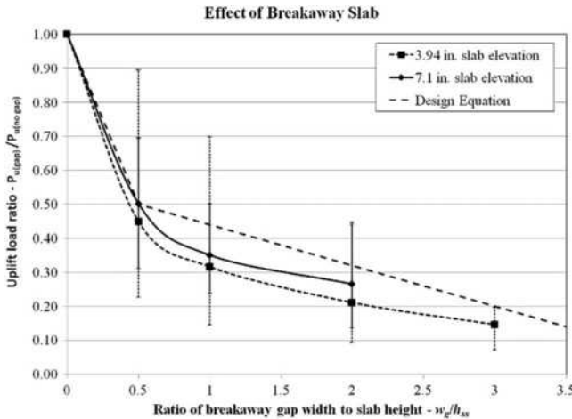
FIGURE C6.10-6 Reduction in Slab Uplift Pressure Caused by Presence of Opening Gap or Breakaway Slab (1 in. = 25.4 mm)
