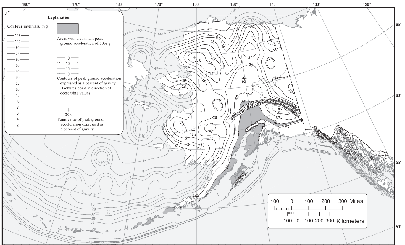
FIGURE 22-10 Maximum Considered Earthquake Geometric Mean (MCE G ) PGA for Alaska
