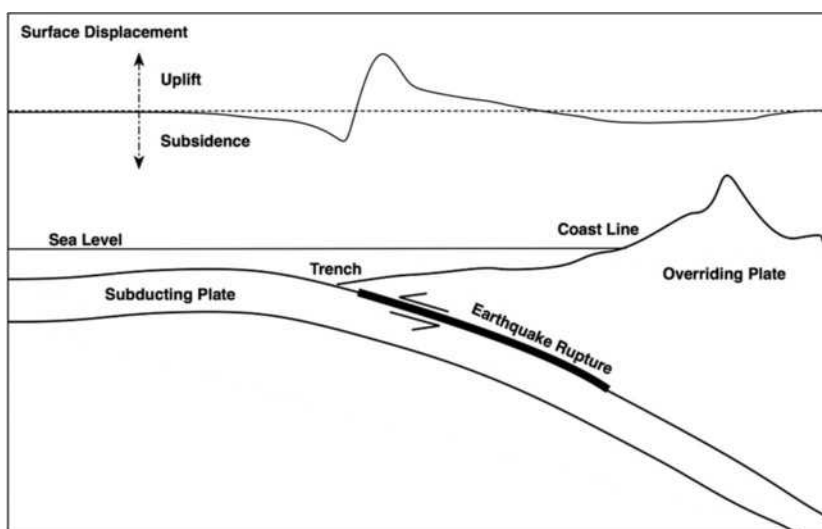
FIGURE C6.7-2 Subduction Zone Earthquake Mechanism for Tsunami Generation
