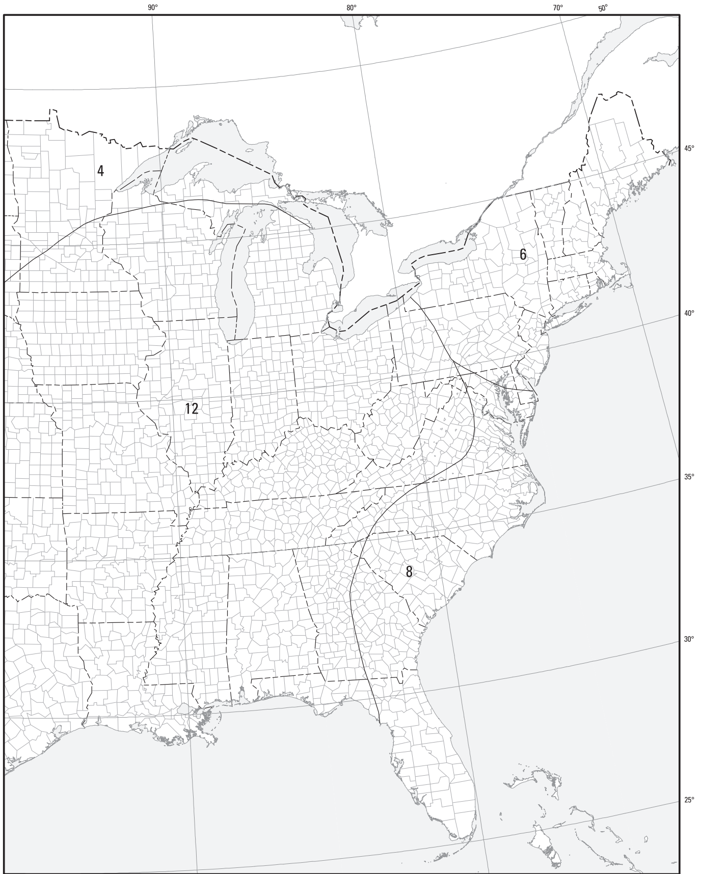
FIGURE 22-14 (Continued). Mapped Long-Period Transition Period, T_L (s), for the Conterminous United States
