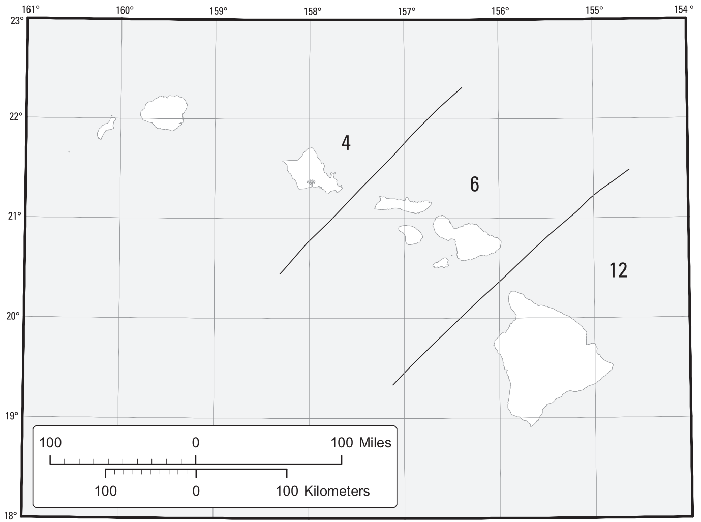
FIGURE 22-16 Mapped Long-Period Transition Period, T_L (s), for Hawaii
