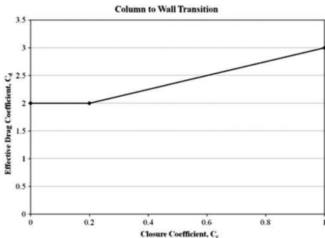
FIGURE C6.10-2 Hydrodynamic Drag Transition from Individual Column to Solid Wall
