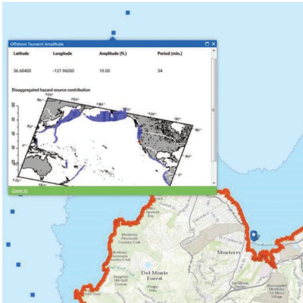
FIGURE C6.7-1 Example of the Offshore Tsunami Amplitude from the ASCE Tsunami Design Geodatabase (amplitude in feet, period in minutes)
