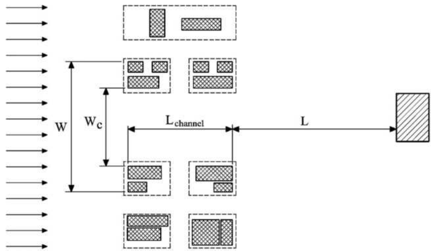
FIGURE C6.8-1 Flow Amplification for Channelized Conditions
