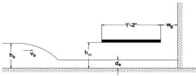
FIGURE C6.10-5 Test Setup to Study Effect of Opening Gap or Breakaway Slab on Uplift Pressure
