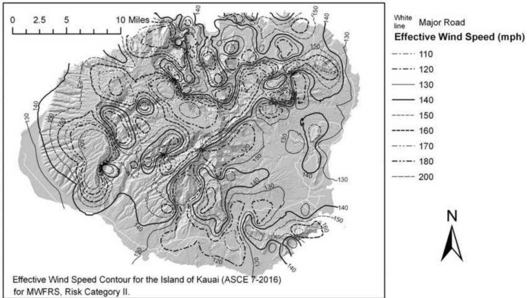
FIGURE 26.5-2B (Continued). Basic Wind Speeds for Risk Category II Buildings and Other Structures: Hawaii
