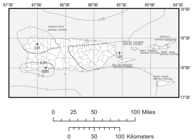
FIGURE 22-19C (Continued) Mapped Risk Coefficient at 1.0-s Spectral Response Period, C_{R1} : Alaska (top), Hawaii (left), Puerto Rico, and U.S. Virgin Islands (right)
