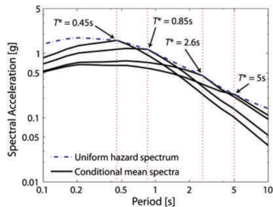
FIGURE C16.2-1 Example Conditional Mean Spectra for a Palo Alto Site Anchored for 2% in 50-Year Motion at T = 0.45s , 0.85s , 2.6s , and 5s
