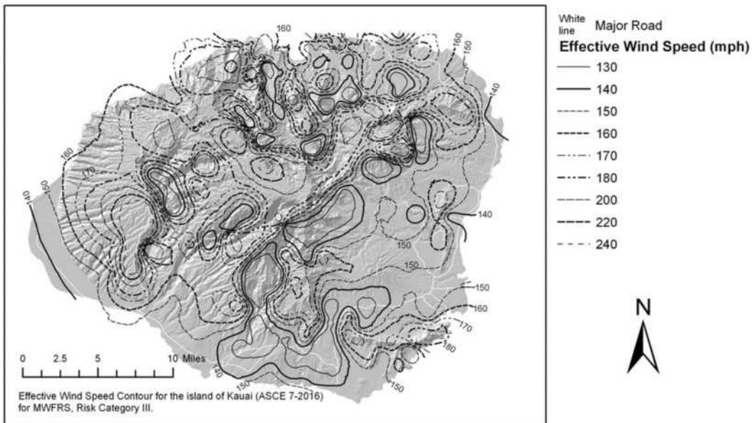
FIGURE 26.5-2C (Continued). Basic Wind Speeds for Risk Category III Buildings and Other Structures: Hawaii
